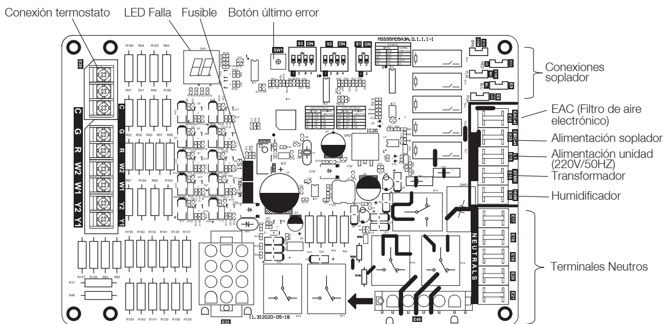
Fig. 26 - Control del calefactor
