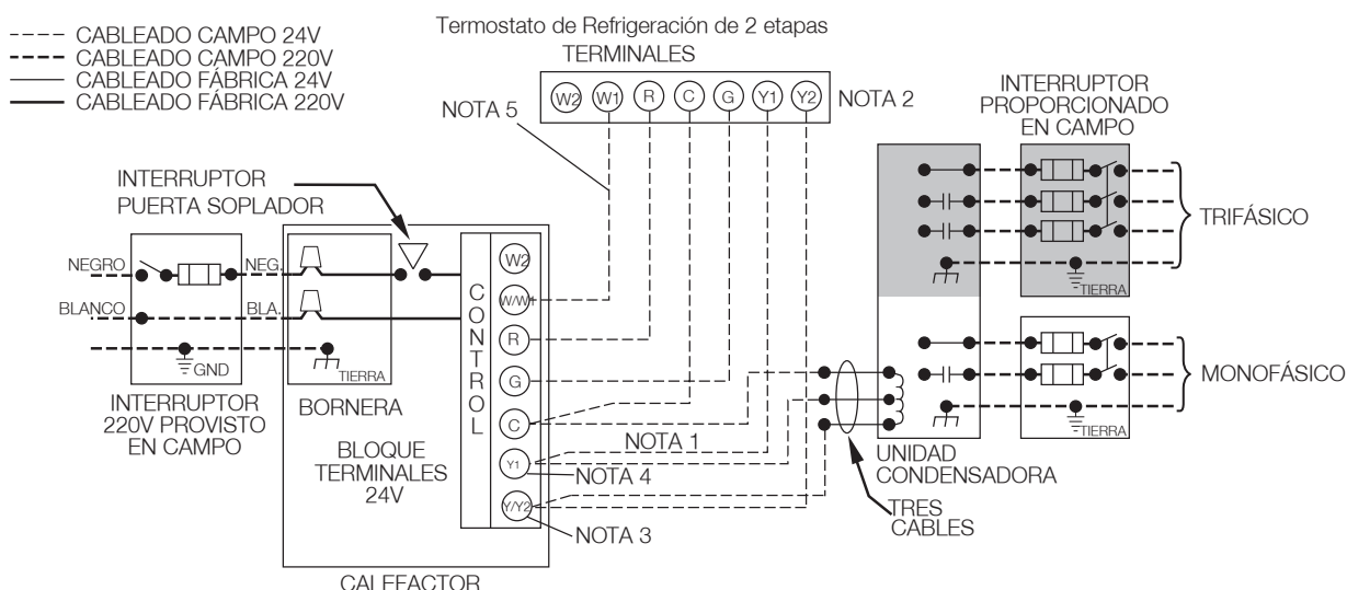
Fig. 26 - Control del calefactor
